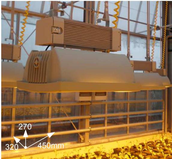
Dimension: 450x320x270mm
